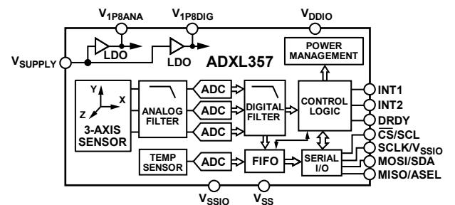
Figure 2. ADXL357
